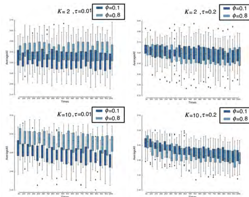
Figure 3: Box-plots of average fitness values of all agents for every 50 time intervals of simulation time span. In this graph, n_g = 80 , HB = 0.6 , and decision rule is "random selection".
