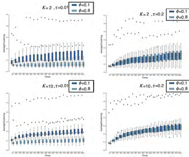
Figure 6: Box-plots of average clustering of the interaction network for every 50 time intervals of simulation time span. In this graph, n_g = 80 , HB = 0.6 , and decision rule is "random selection".
