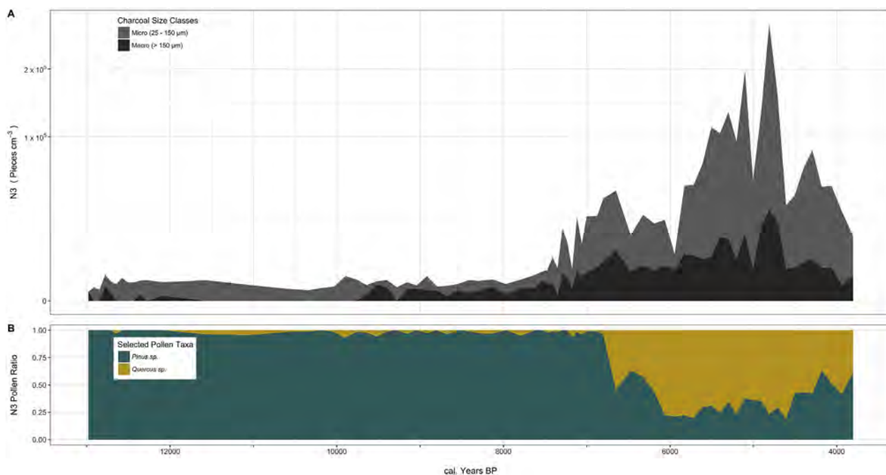
Fig. 4. Summary of N3 sedimentary charcoal record empirical data; A) micro- and macro-charcoal counts (note square root transformation of y-axis to highlight low charcoal counts from 13,000 to 8000 BP); B) ratio of Pinus sp. and Quercus sp. pollen counts from the N3 record.
