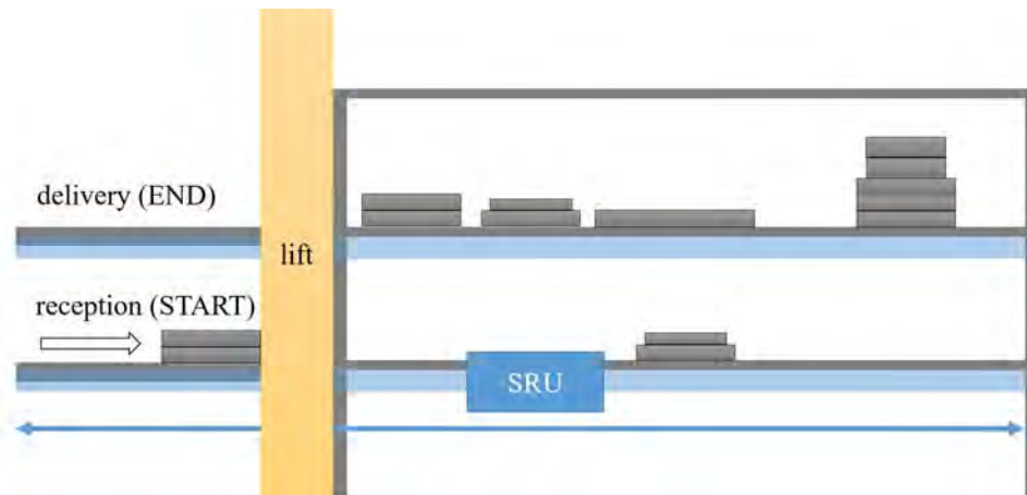
Figure 3: In an early sketch of LOCSys, the system consists of a shuttle with a gripper and a lift to change the height of the storage and retrieval unit.
