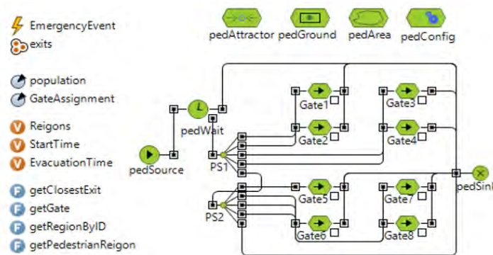
Figure 4: Anylogic Pedestrian Model.
