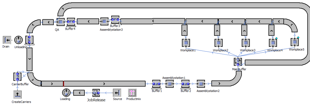
Figure 1: 2D view of the assembly line model.
