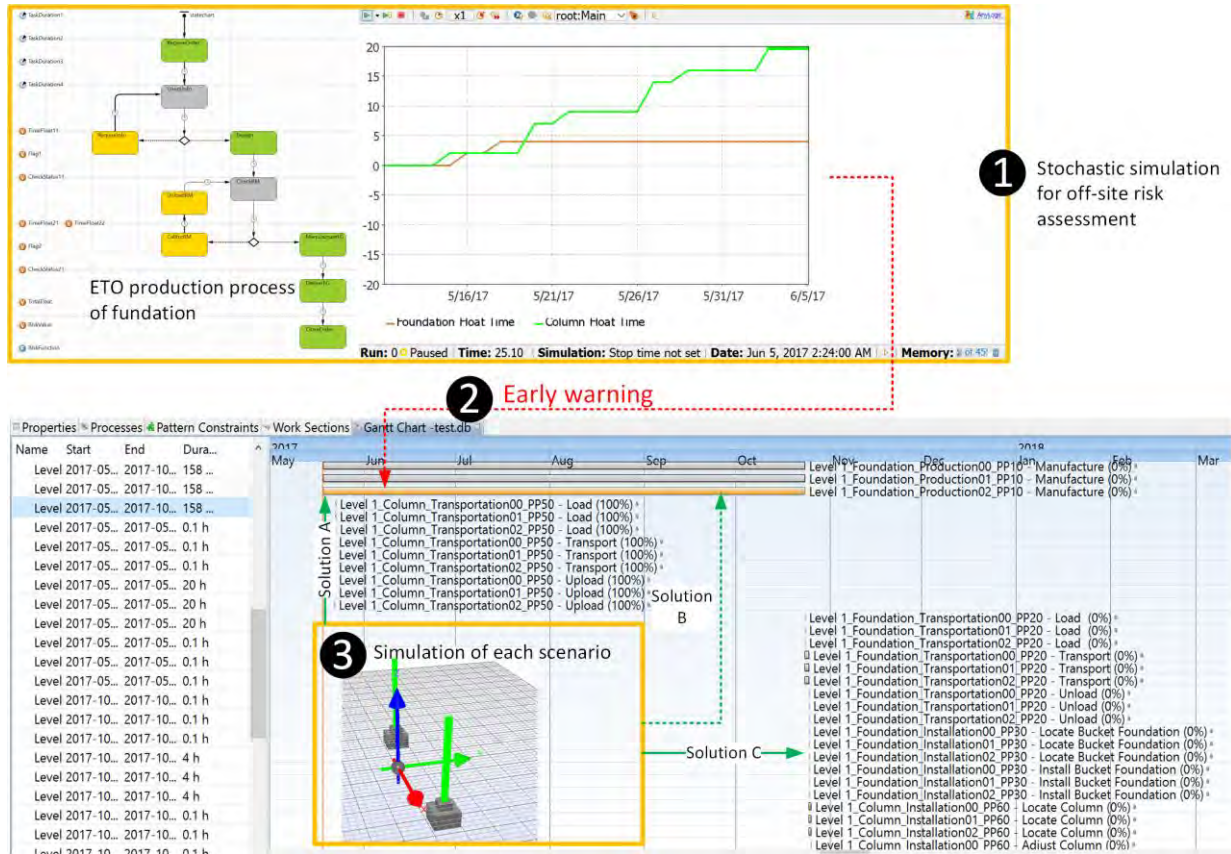
Figure 9: An on- and off-site logistics simulation example of bucket foundation and column.
