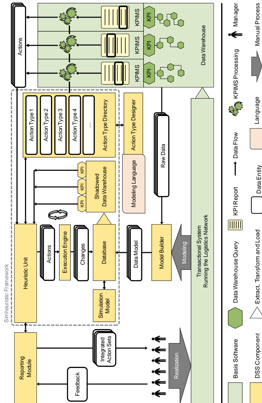
Figure 2: Architecture of the decision support system, based on Rabe and Dross (2014, 2015, 2017a).
