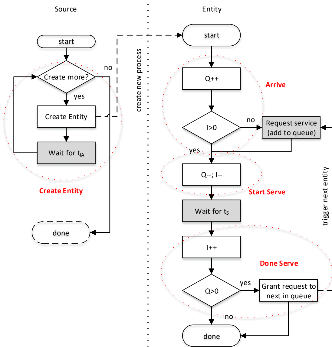
Figure 3: Process flowchart representation of M/M/n queuing system.
