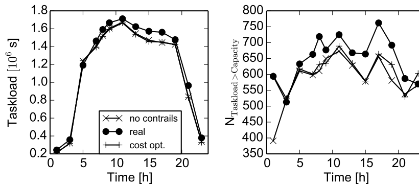
Figure 5: Left: Sum of controller's taskload per hour over the day. Right: Number of air spaces where taskload exceeds capacity, as measure of air space complexity. Both optimized scenarios show a better distribution of aircraft and taskload to the European airspace. Therewith, the airspace complexity could be reduced by considering individual aircraft performance in a 4D waypoint free trajectory optimization.
