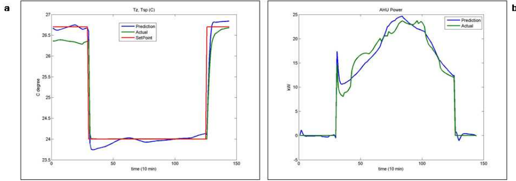
Figure 3: NARX model prediction: (a) zone temperature (b) zone power.
