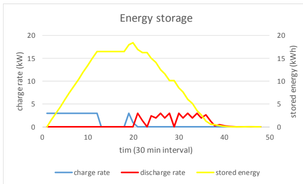
Figure 5: Charge, discharge, storage of ESS.
