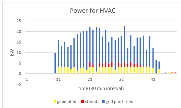
Figure 6: Energy for powering HVAC.
