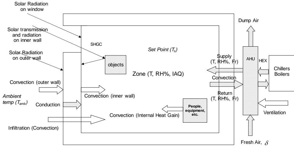
Figure 1: Schematic view of heat transfer in a building.
