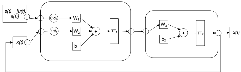
Figure 2: NARX model for thermal behavior of building.
