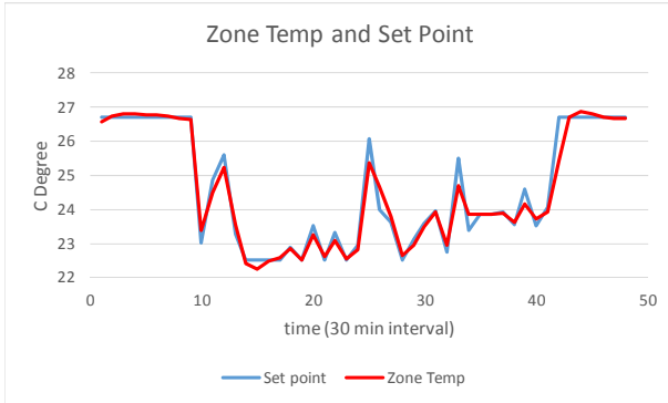
Figure 3: Optimal set point and zone temperature.
