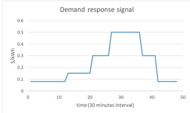
Figure 4: Demand response signal.
