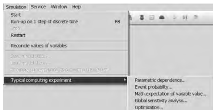
Fig. 6. RMD’s tools for computing experiments
