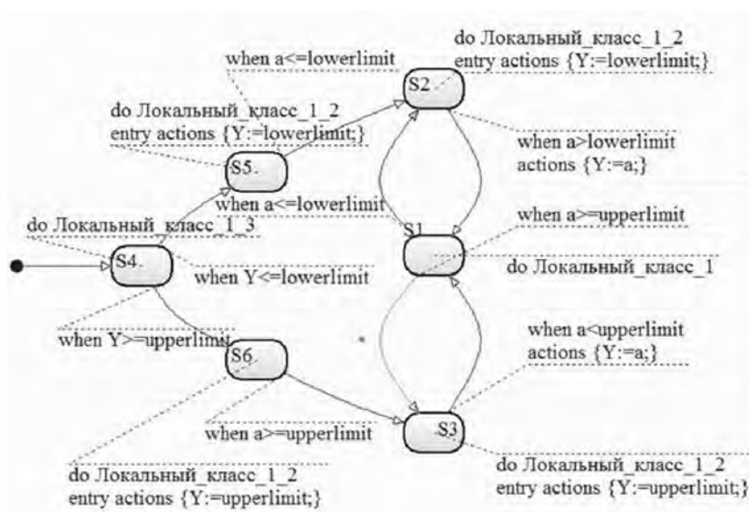
Fig. 14. RMD's "Integrator" simulator
