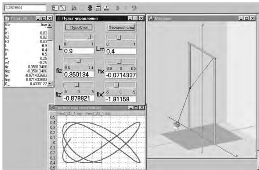
Fig. 12. Professor S.V. Biryukov's model — a test bench for schools
