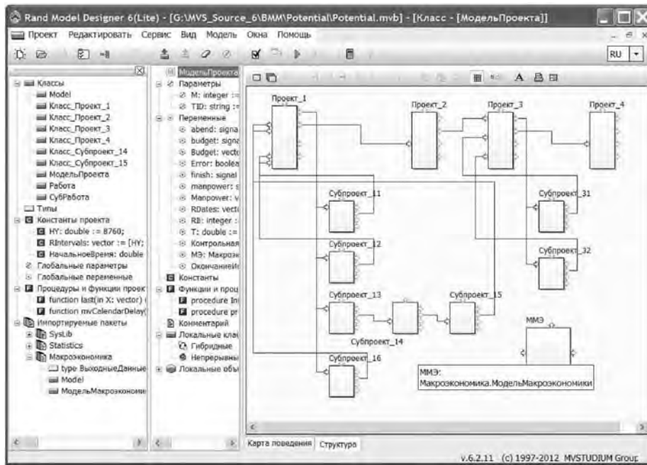
Fig. 11. RMD's macroeconomic model
