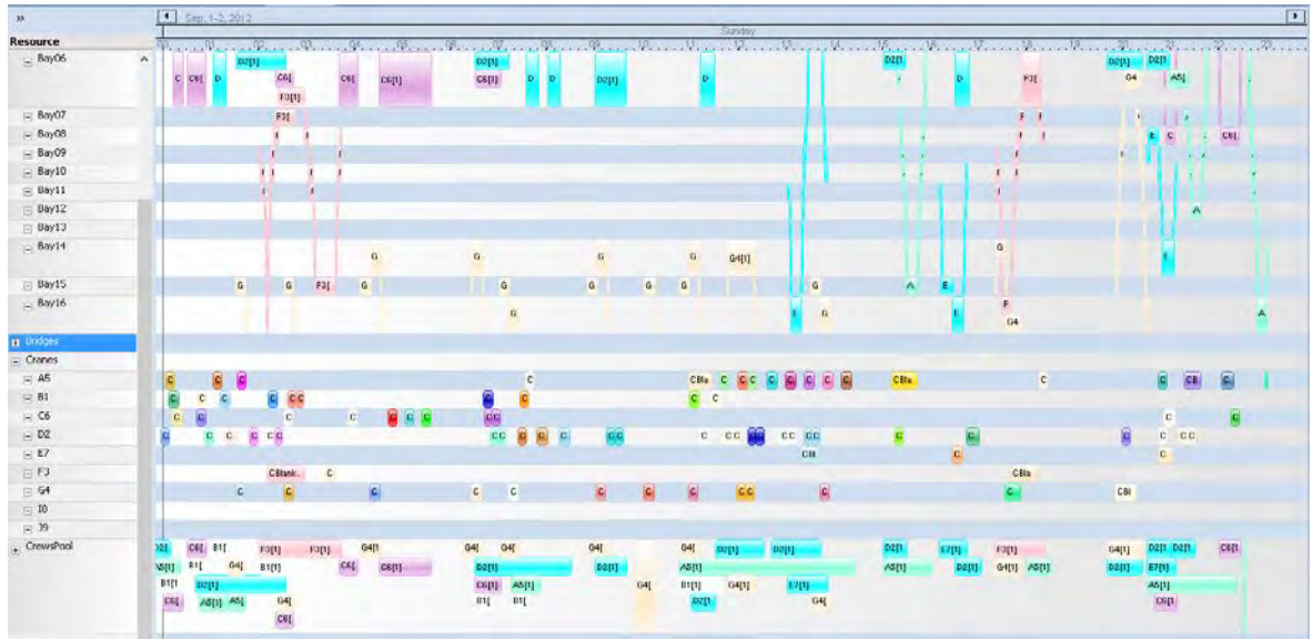
Figure 7: Gantt chart showing resource usage during a model run, including cabs and bays.
