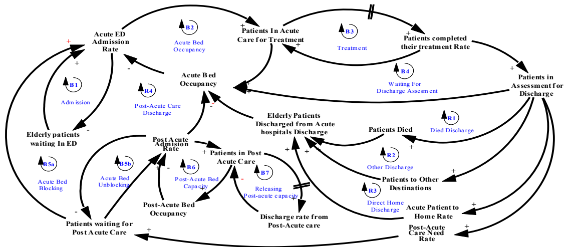
Figure 1: Simplified Causal Loop Diagram for Elderly Patients' Bed Blocking
