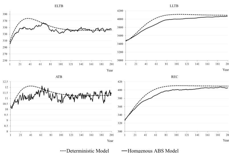
Figure 7: Aligning the homogenous ABS model against the deterministic model.
