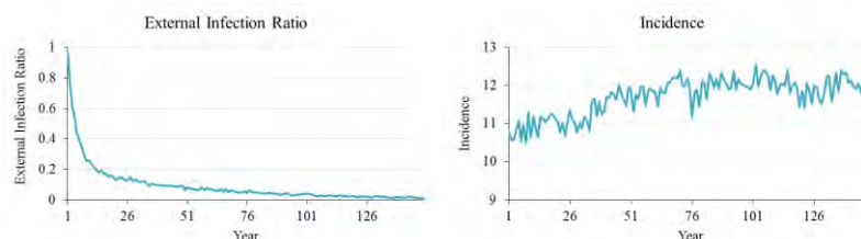
Figure 2: ABS output patterns.
