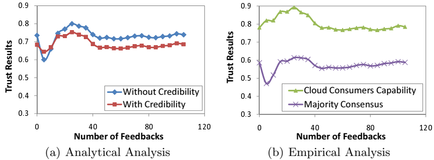
Fig. 2. Experimental Evaluation
