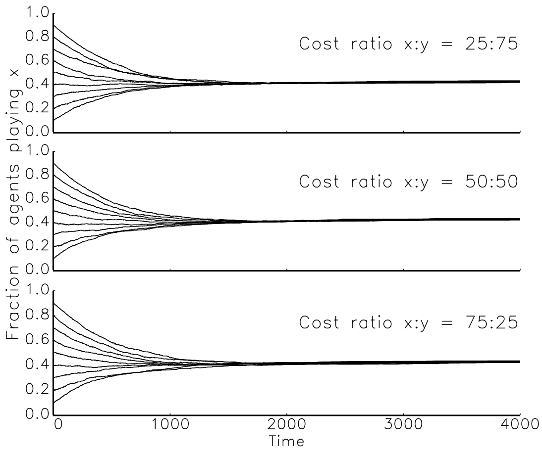
Figure 6: Degree two, substitutes, cost ratios compared.
