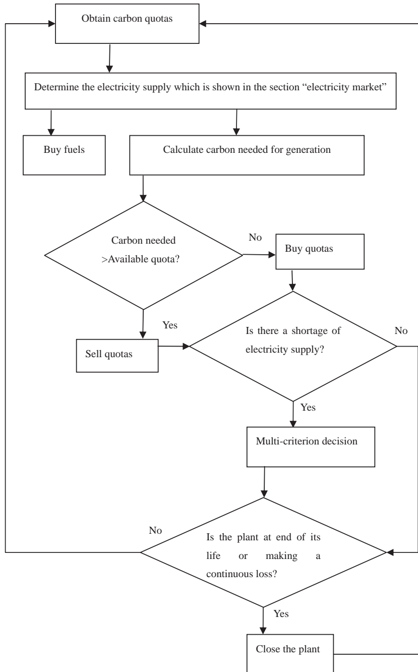
Fig. 2. Flow chart of power producers' actions.
