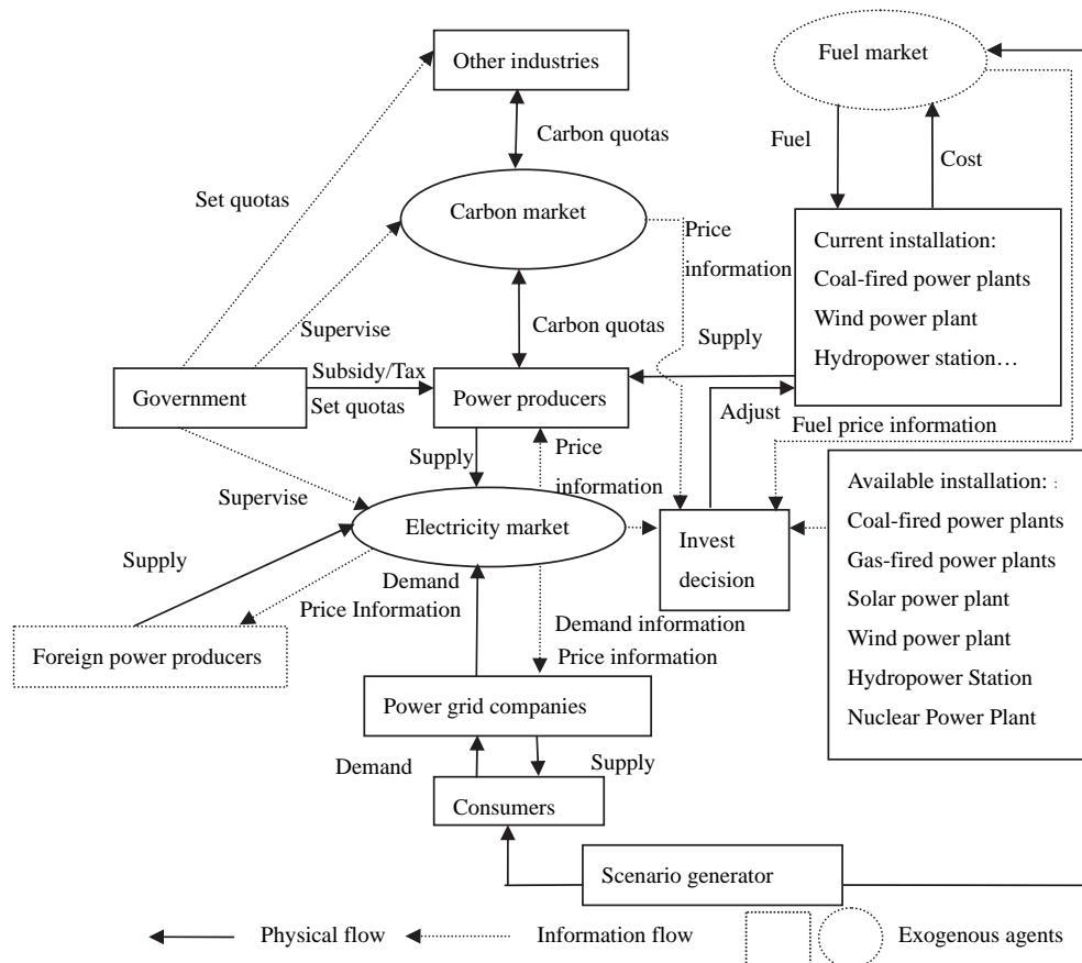
Fig. 1. System structure.
