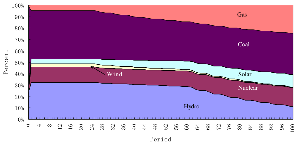
Fig. 6. Power source structure when CET is not introduced.
