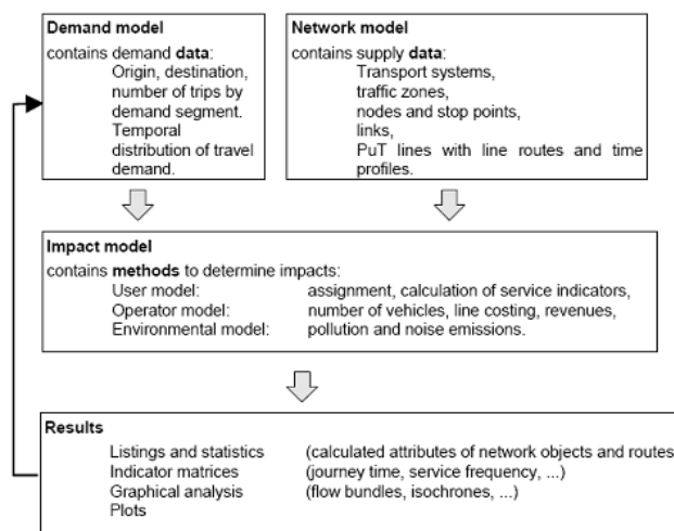
Figure 4. VISUM transport model [7]
