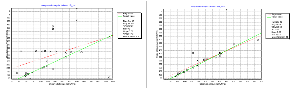
Figure 9. Dependence between simulated and real flow distribution before and after calibration
