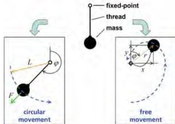
Figure 9. Sketch of string pendulum
