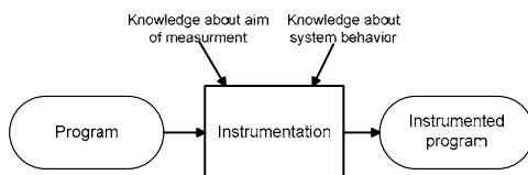
Figure 4: Program Instrumentation
