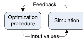
Figure 1: Simulation-Based Optimization
