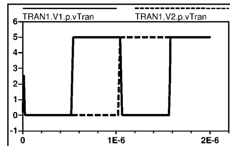
Figure 16: Input stimuli (equal for both gates).
