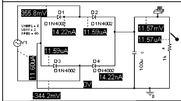
Figure 9: OP analysis results. SPICELib using SMI algorithm (above). ORCAD PSpice (below).
