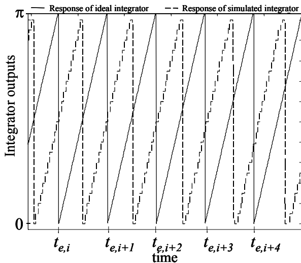
Figure 2: Integrator Outputs
