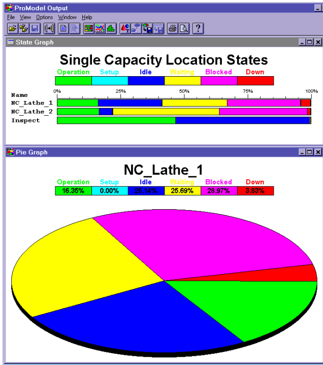
Figure 5: A Location State Graph
