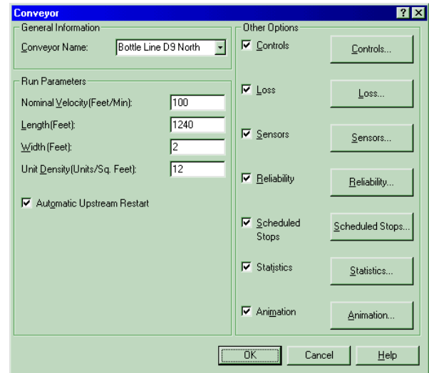
Figure 5: Conveyor Dialog from Arena Packaging
